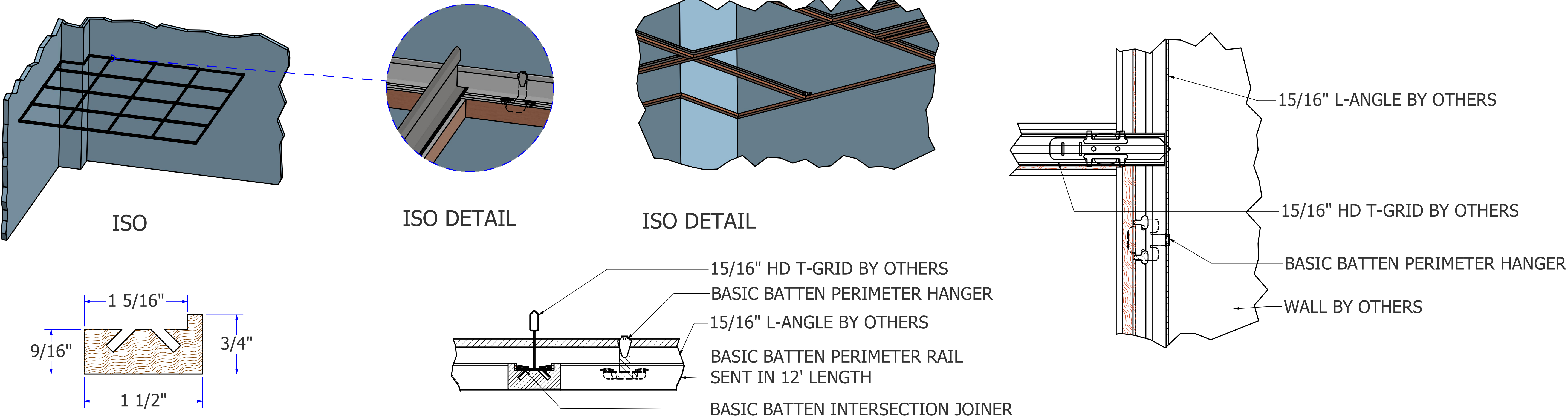
SIDE VIEW - CONNECTION TO BASIC BATTEN PERIMETER RAIL
