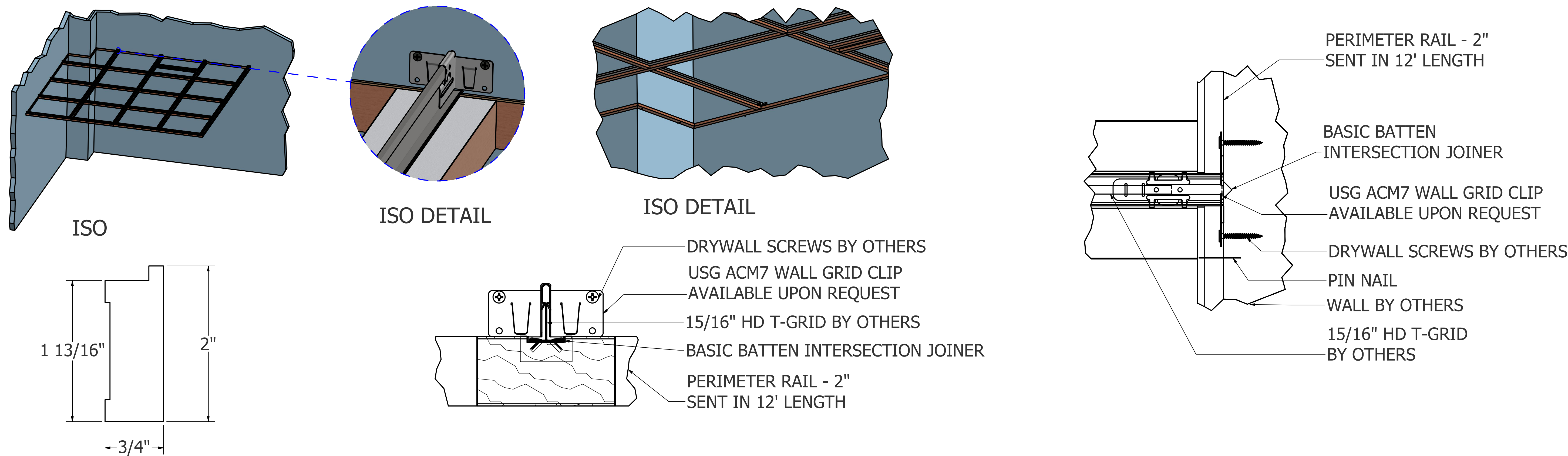
END VIEW - PERIMETER RAIL 2"
