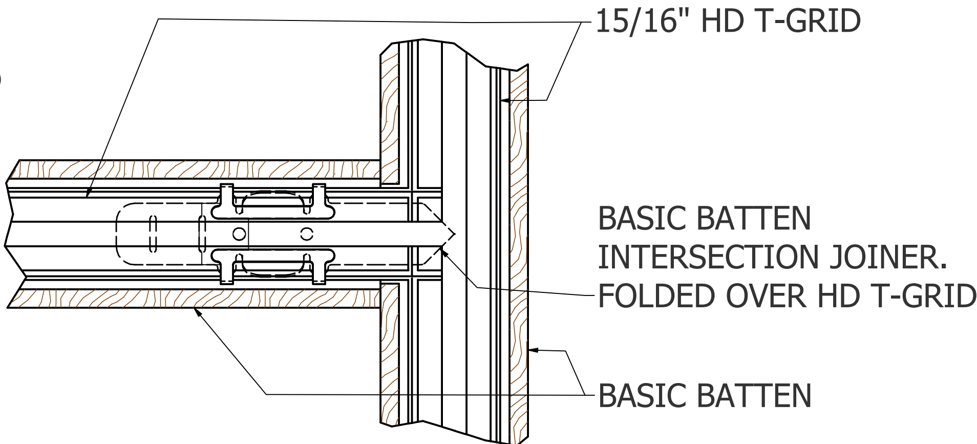
E PLAN VIEW - BUTT JOINT
