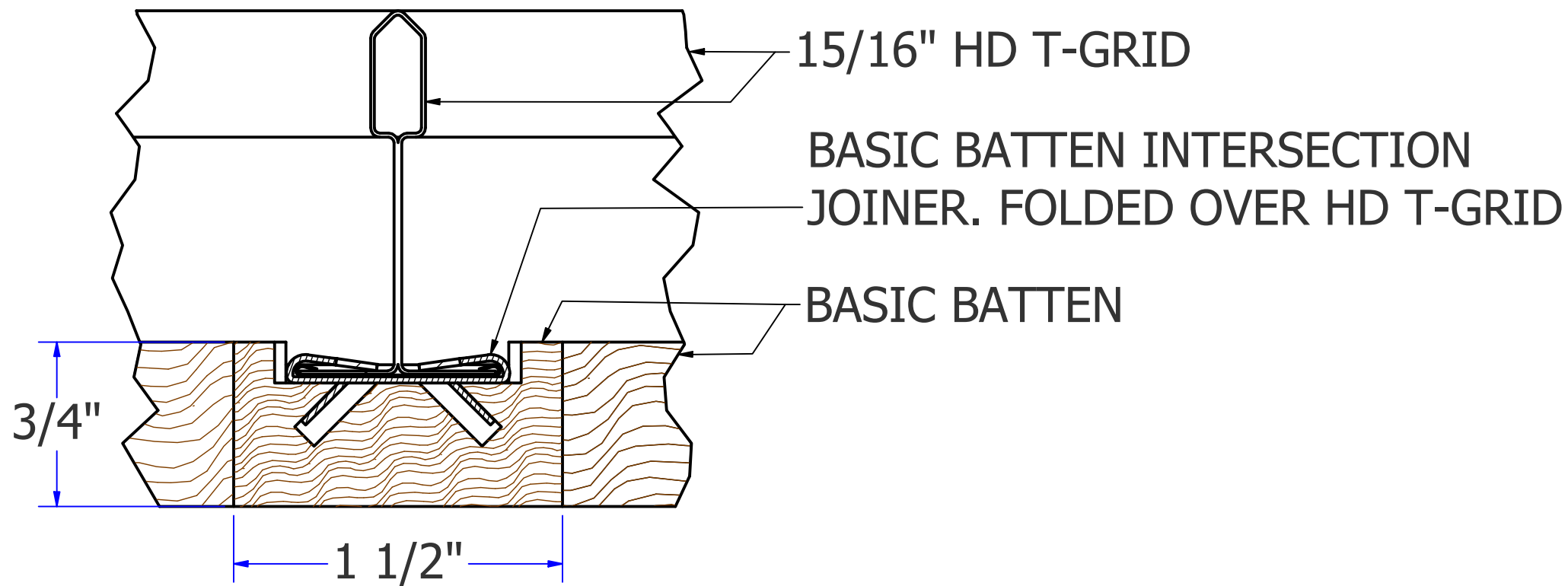
D END VIEW - BUTT JOINT
