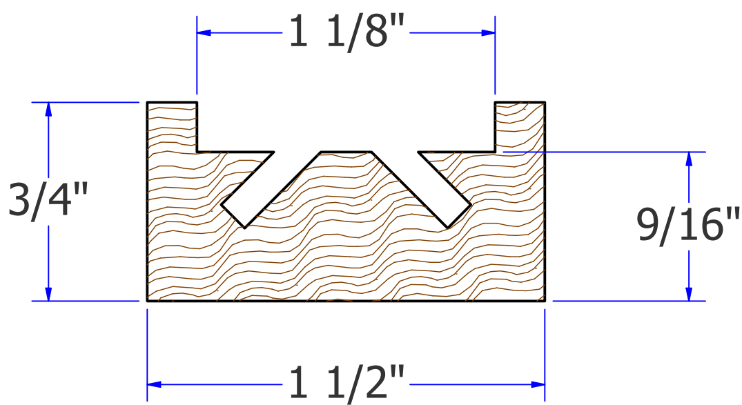
END VIEW - BASIC BATTEN
