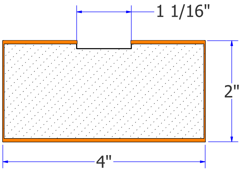
END VIEW - ACOUSTIC BATTEN
