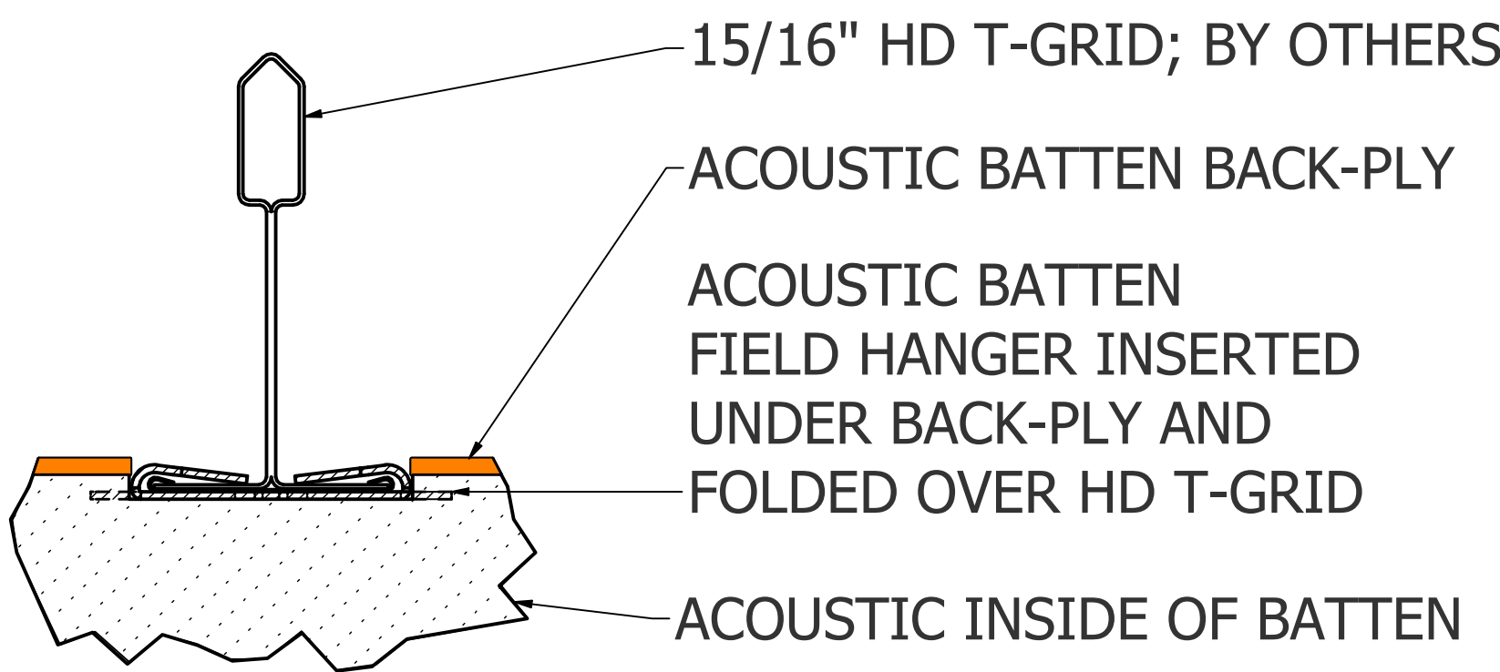
B END VIEW - CONNECTION TO HD T-GRID
