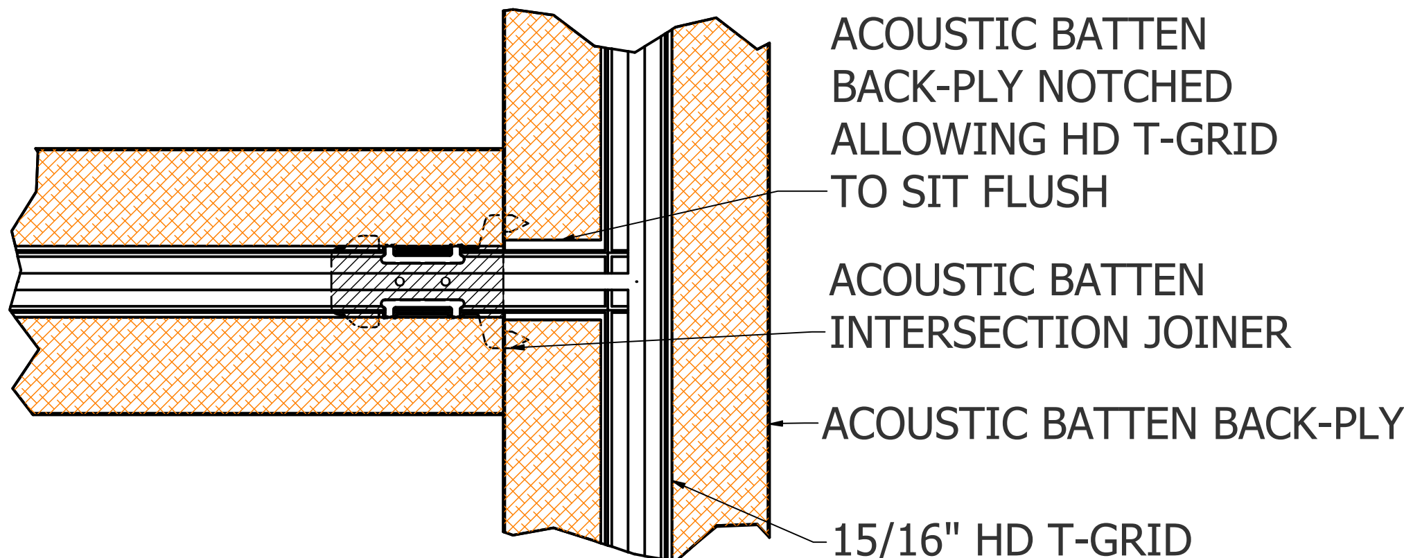
E PLAN VIEW - BUTT JOINT
