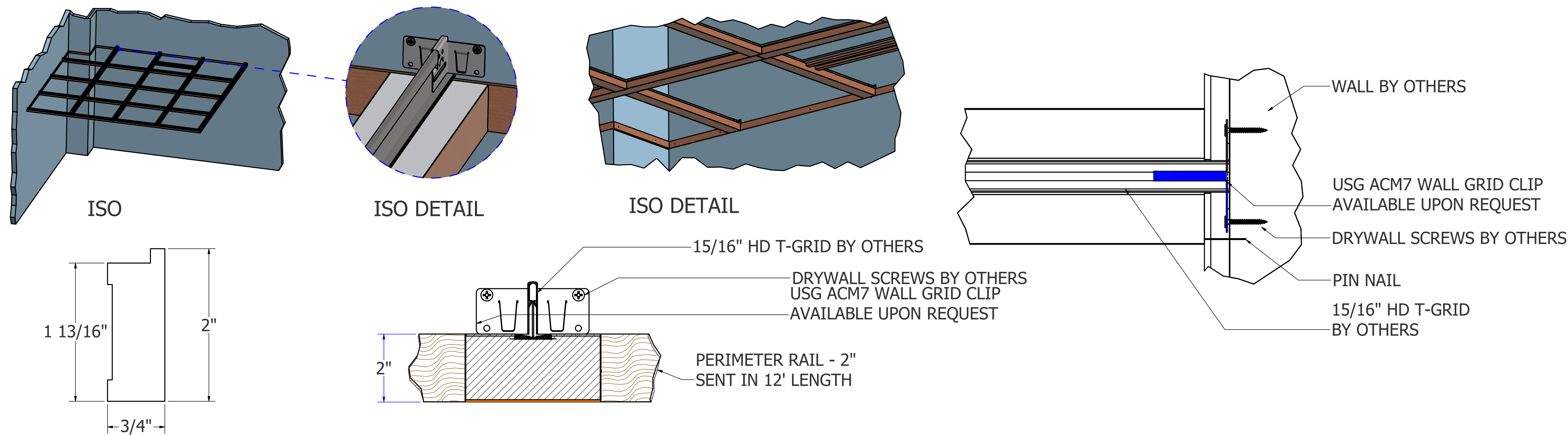
END VIEW - PERIMETER RAIL 2"
