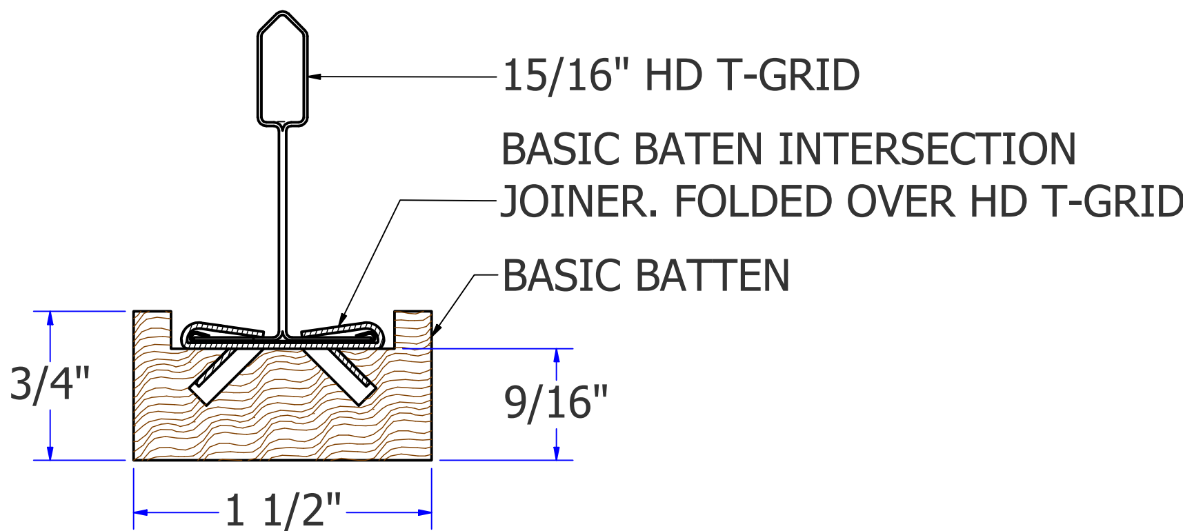
B END VIEW - CONNECTION TO HD GRID
