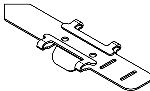
Basic Batten Intersection Joiner H106-1395
