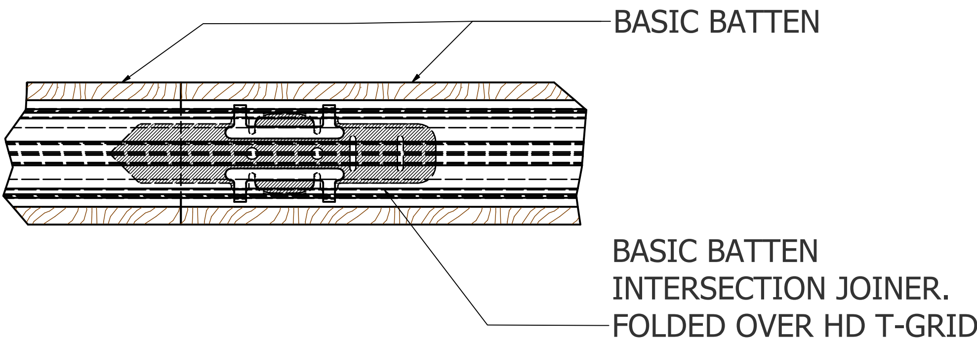
PLAN VIEW - BASIC BATTEN EXAMPLE
