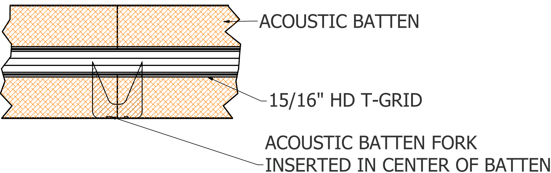
A PLAN VIEW - END TO END ACOUSTIC BATTENS
