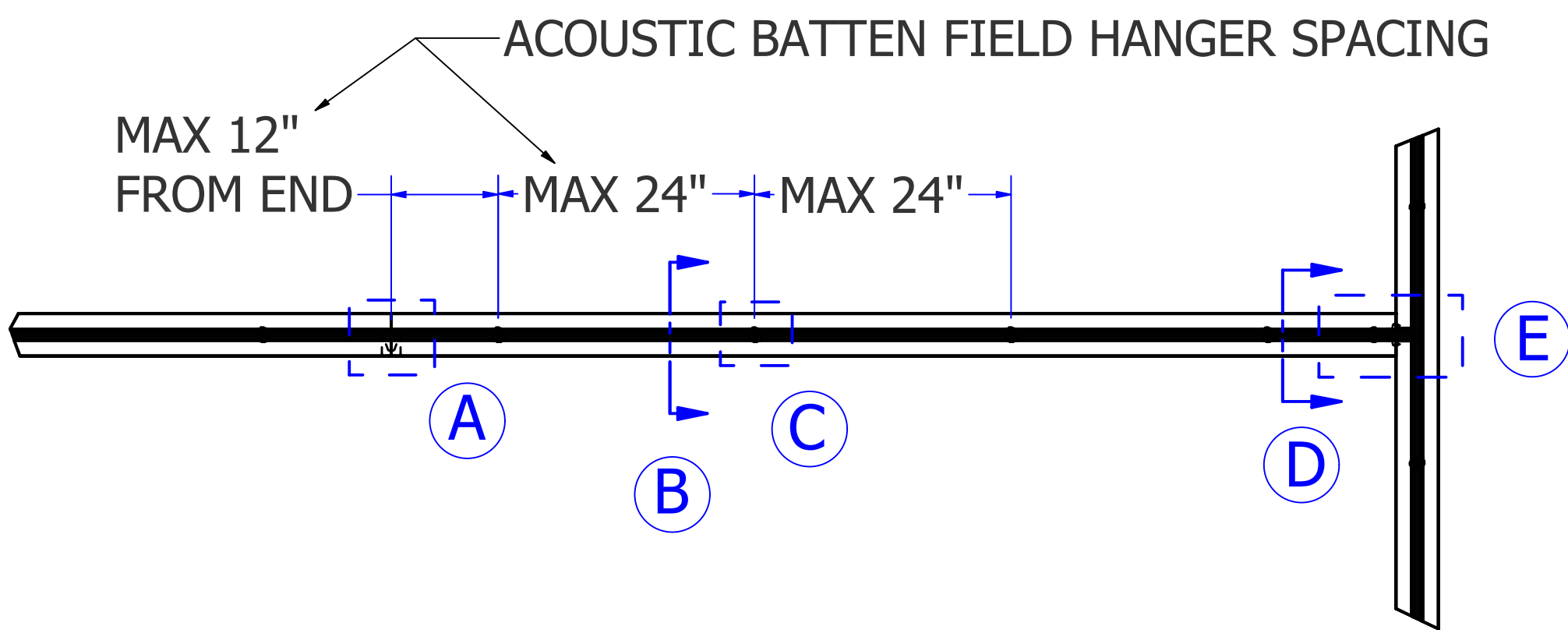
PLAN VIEW - ACOUSTIC BATTEN EXAMPLE
