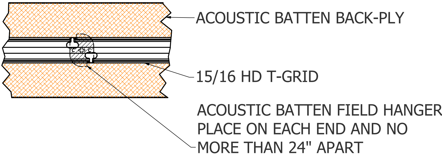
C PLAN VIEW - CONNECTION TO HD T-GRID
