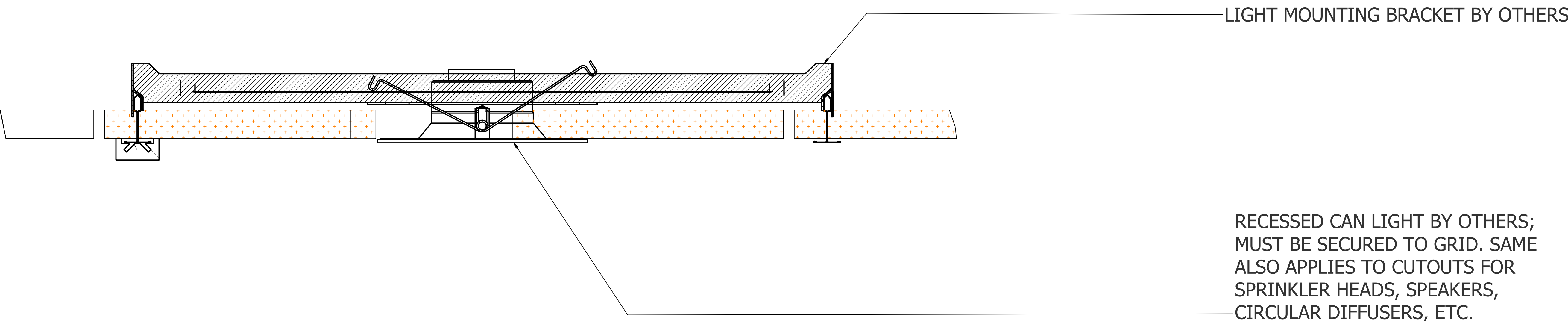
SECTION VIEW - INSET PANEL CUTOUT
