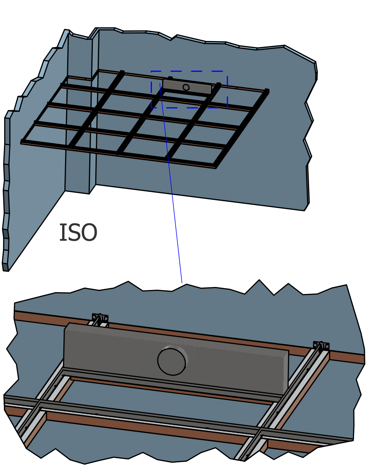
ISO ISO DETAIL
