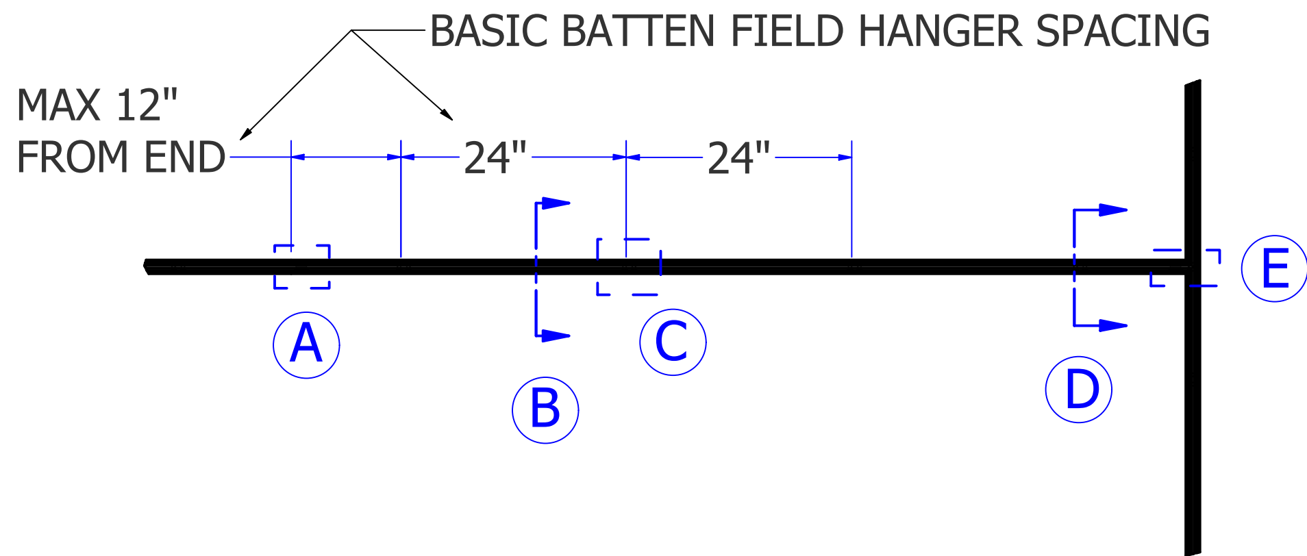
PLAN VIEW - BASIC BATTEN EXAMPLE
