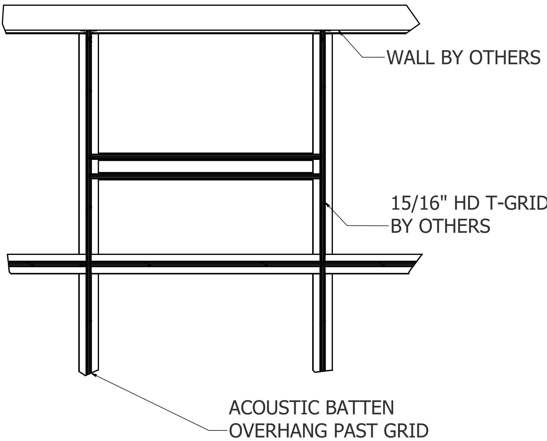
PLAN VIEW - PANEL CUTOUT
