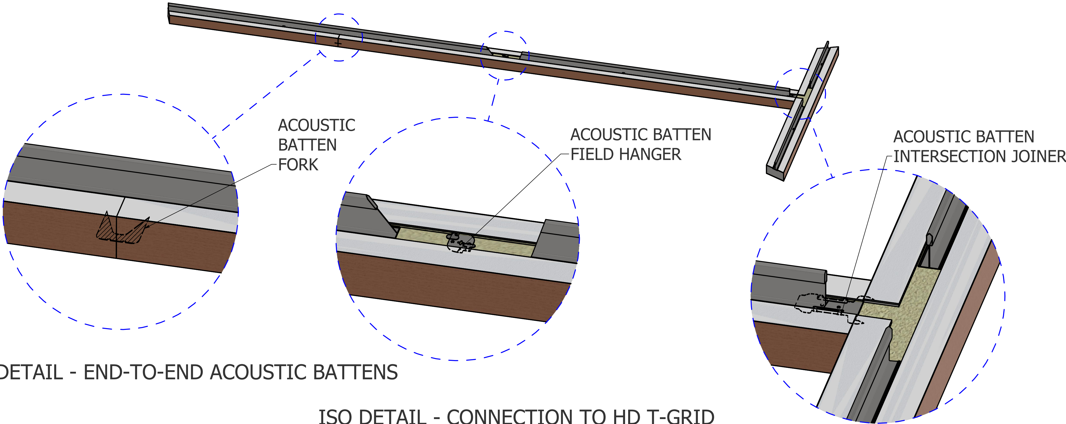
ISO DETAIL - BUTT JOINT
