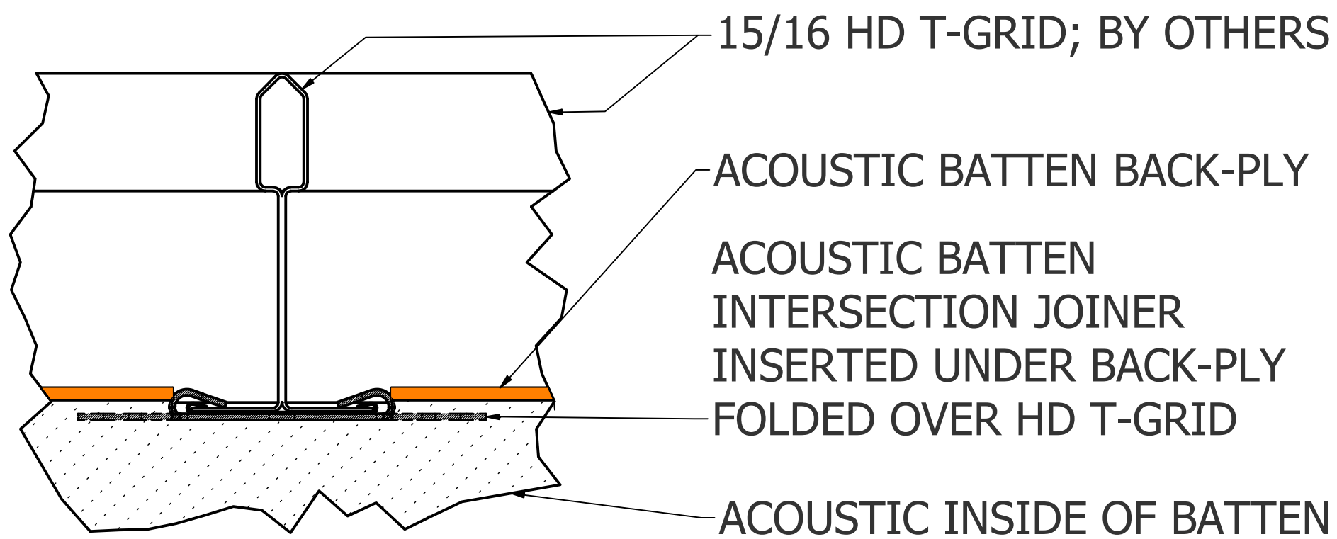
D END VIEW - BUTT JOINT
