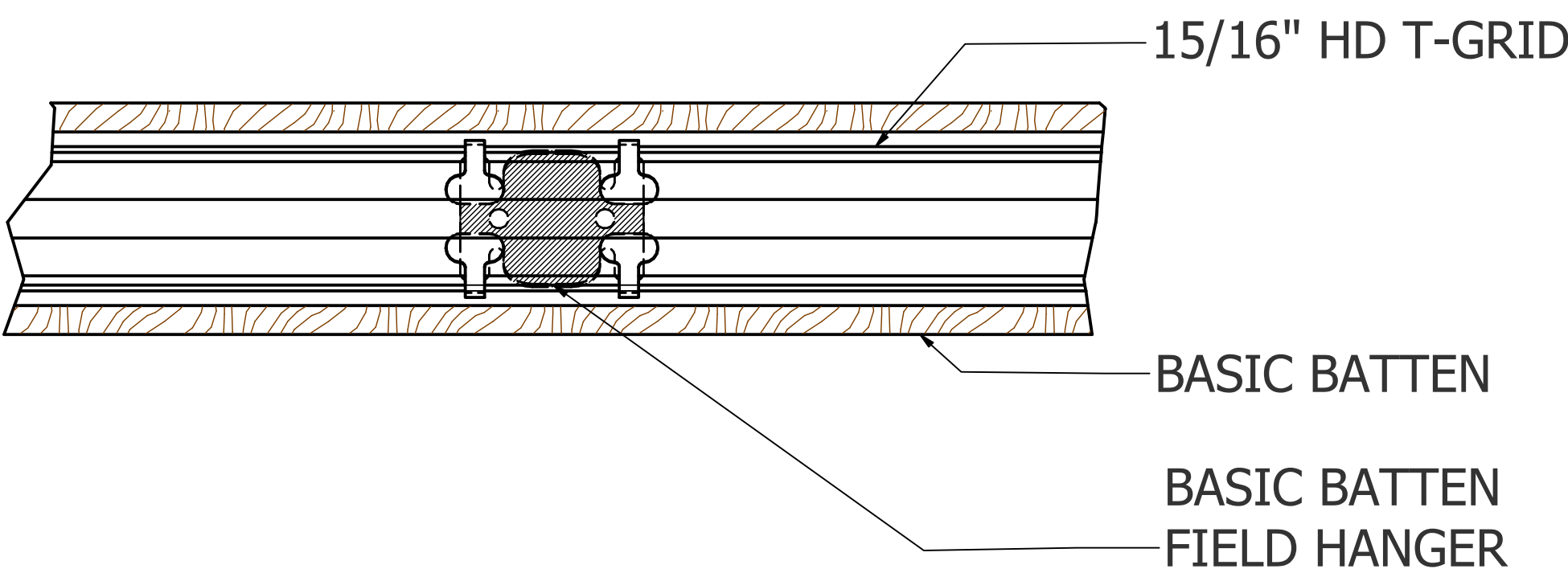
C PLAN VIEW - CONNECTION TO HD GRID
