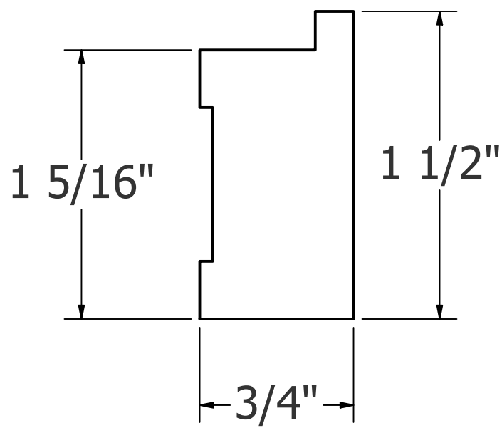
END VIEW - PERIMETER RAIL 1 1/2"
